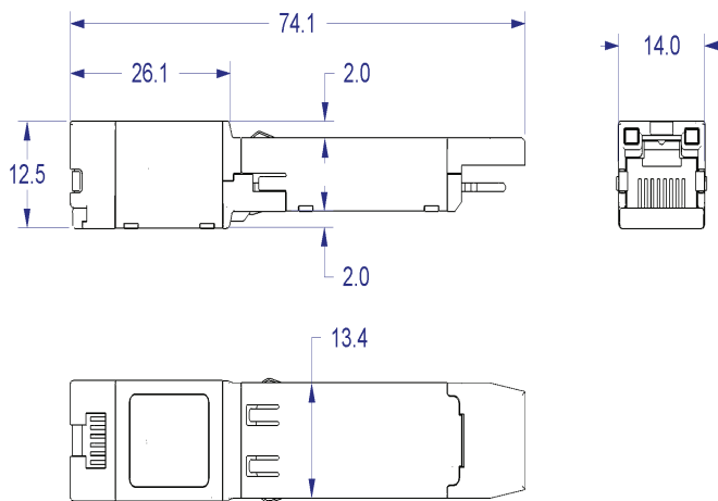
Figure 2 Physical Dimensions
